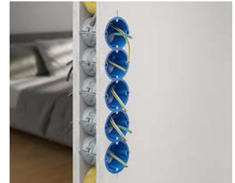
The sound insulation box can be used in up to five opposing combinations without weakening the sound insulation characteristics of the wall.
