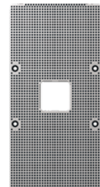
Universal mounting plate with broken-out exit for luminaires.
